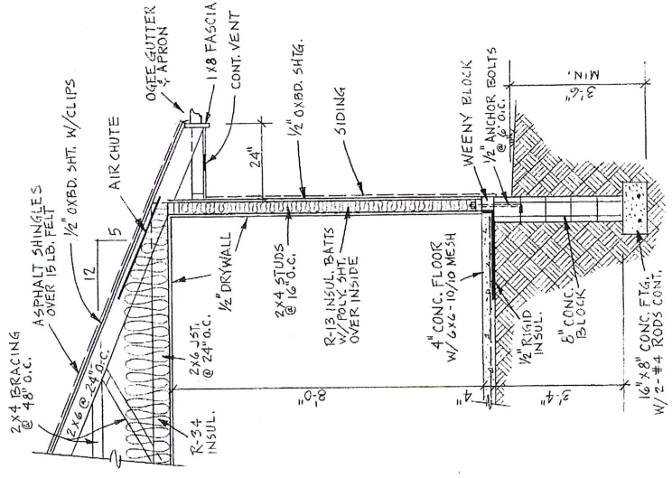
TYPICAL SECTION 1/2" = 1'-0"
