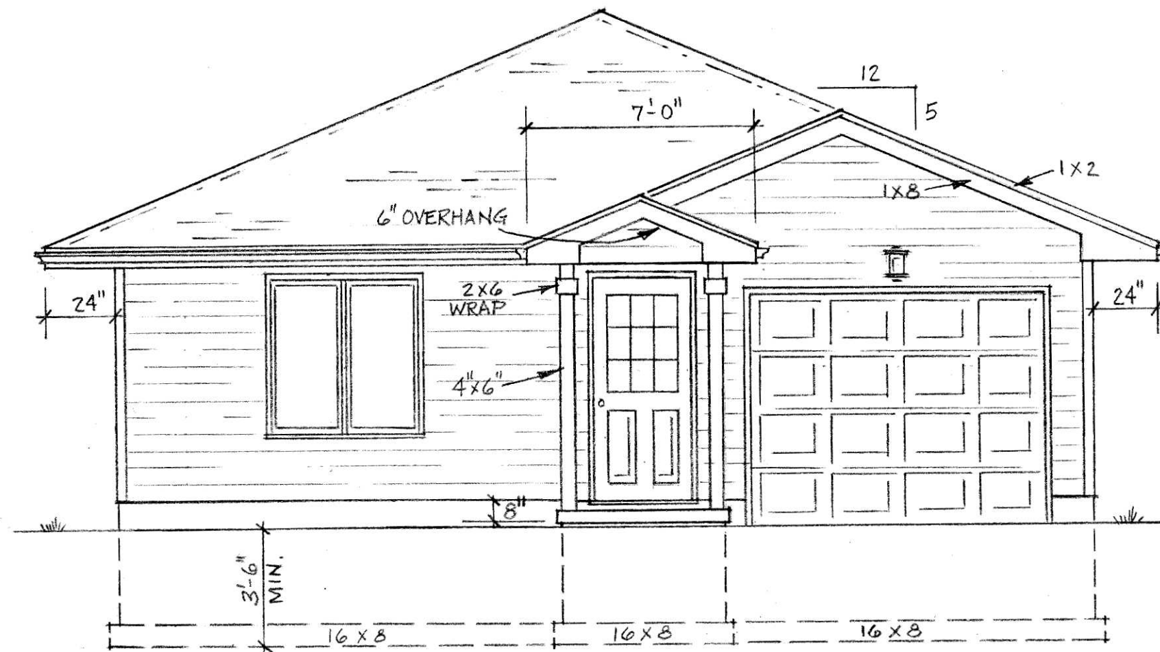
FRONT ELEVATION 1/4" = 1'-0"
