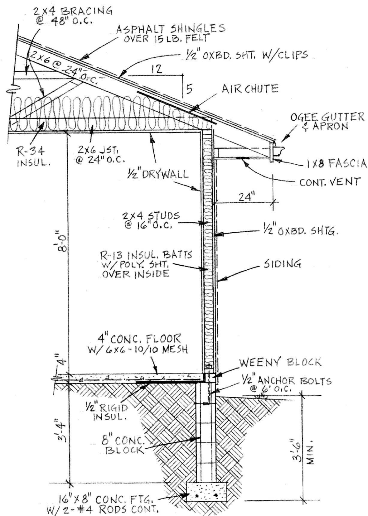
TYPICAL SECTION 1/2" = 1'-0"
