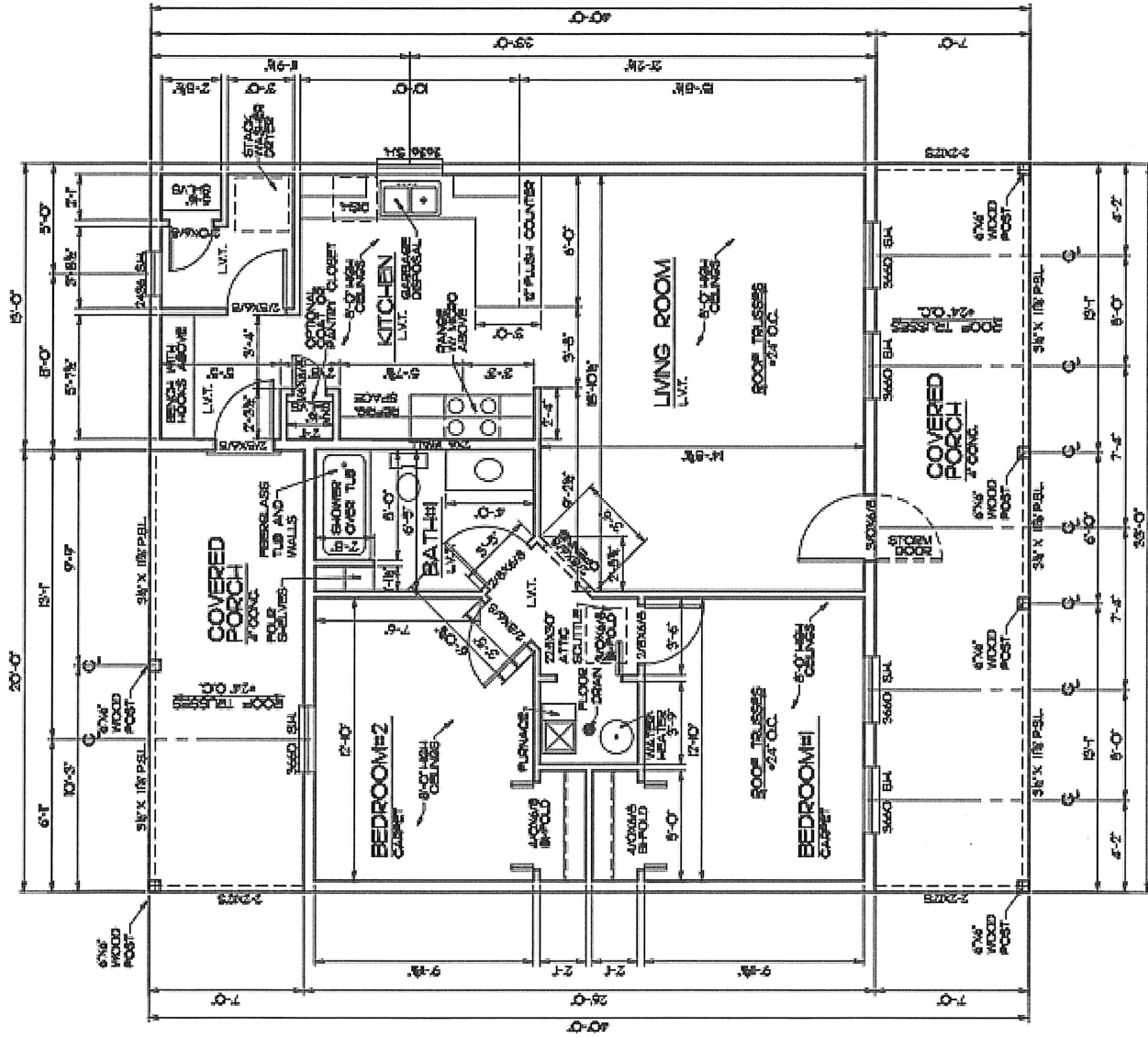
FIRST FLOOR PLAN FIRST LEVEL - 948 SQ. FT. SCALE 1/8" = 1'-0"
